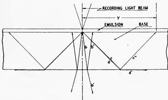
FIG. 13. Illustration of reflection at critical angle of light scattered by the emulsion.
